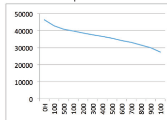
Lumen Depreciation Curve
