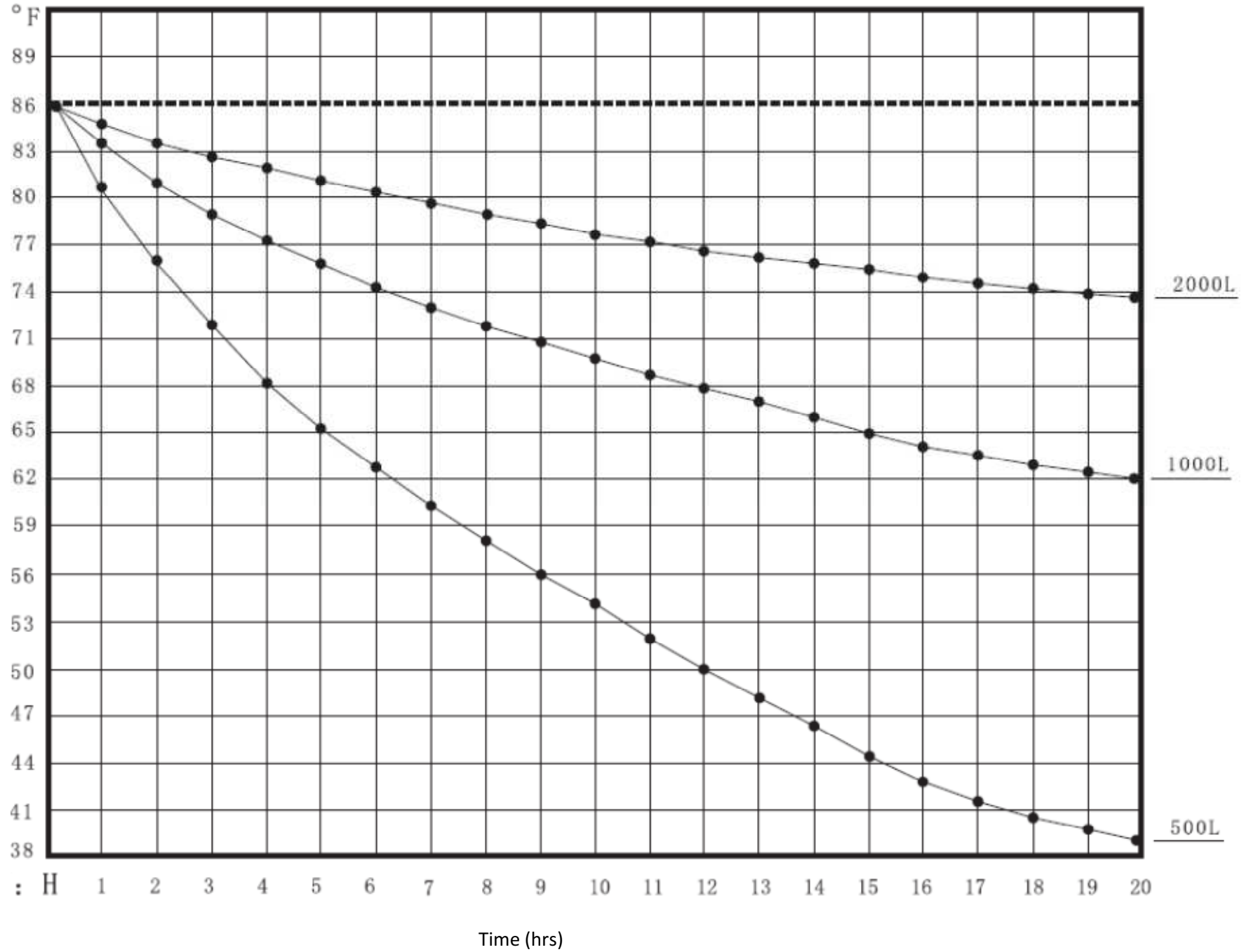
AACH100 Performance Chart. Ambient temperature: 88°F
