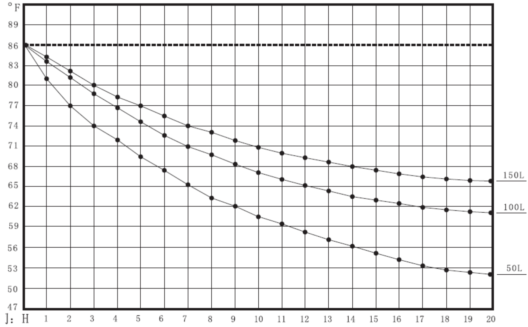
AACH10 Performance Chart. Ambient Temp: 88F, Initial Water Temp 86F
